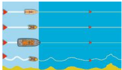
6. Line abreast search
