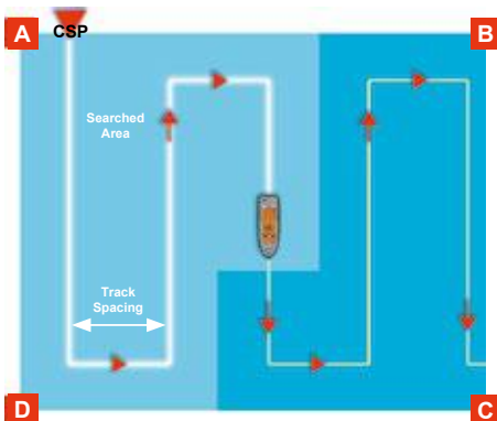
2. Creeping line ahead search
